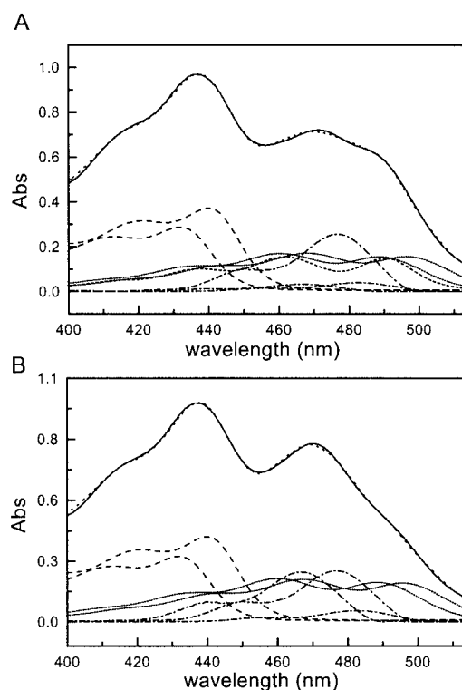
FIGURE 2 Description of the Soret region of the absorption spectra of LHCII-neolute in ( A ) and LHCII-lute in ( B ) in terms of the absorption of single pigments. The absorption spectra of both complexes ( solid line ) are compared with the reconstituted spectra obtained as a sum of the bands of the single pigments ( dotted line ). The spectra of the individual pigments are also shown: Chl a ( dashed line ), Chl b ( dot-dash ), lutein ( short dot ), neoxanthin ( short dash ).
