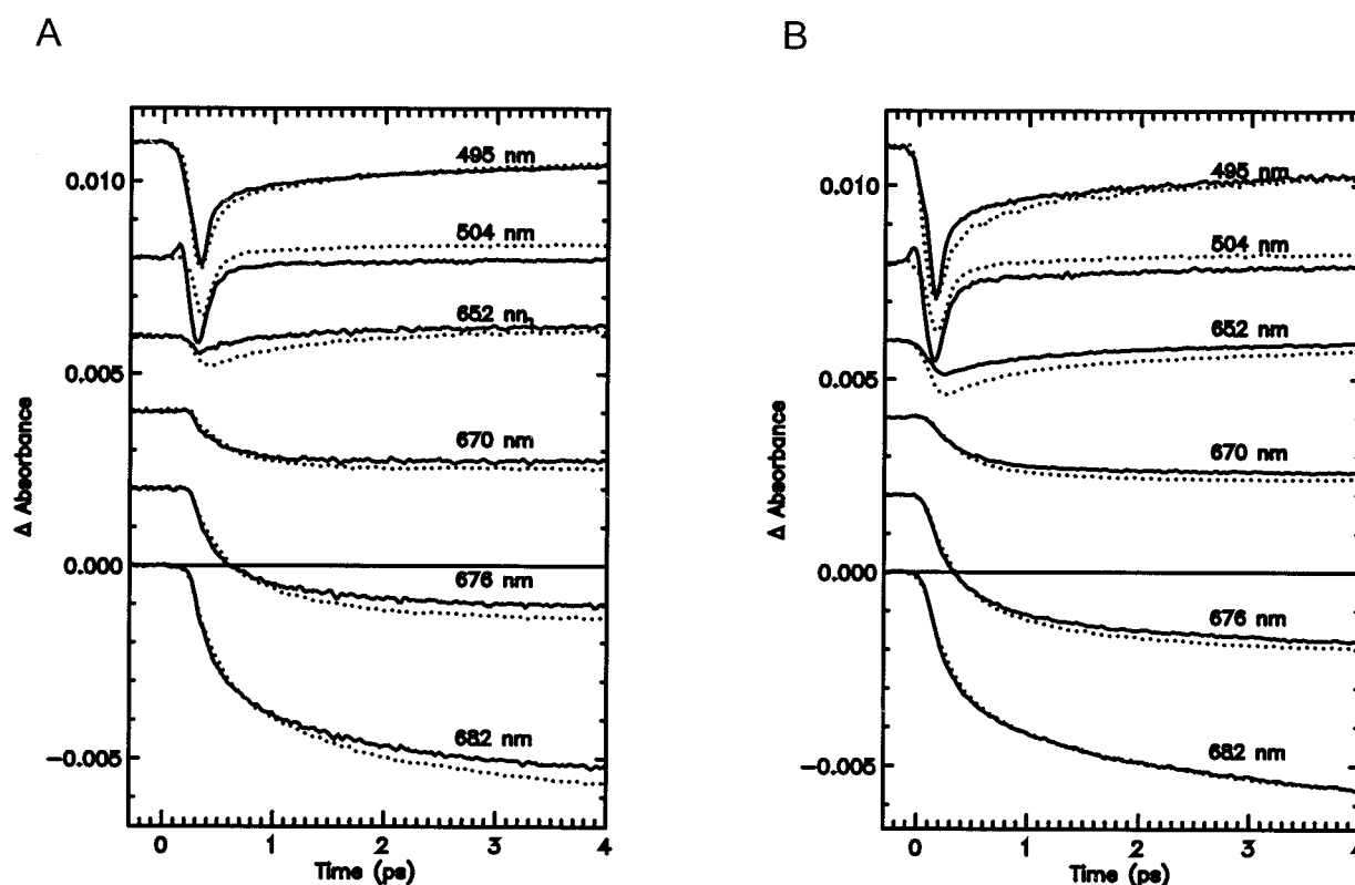
FIGURE 1 Experimental transient absorption kinetics for selected excitation/detection wavelength pairs for LHCII-lutein ( A ) and LHCII-neolutein ( B ). Solid line: excitation at 500 nm; dotted line: excitation at 490 nm.
